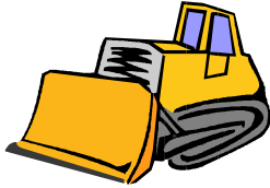
bulldozer
