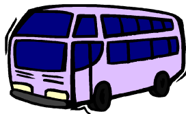
bus
